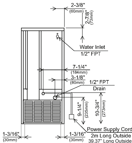
AM-50BAE/AM-50BAE-DS
