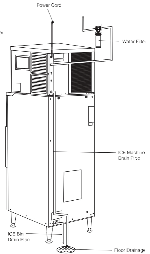
Back View of 194HBN12022 Installation
